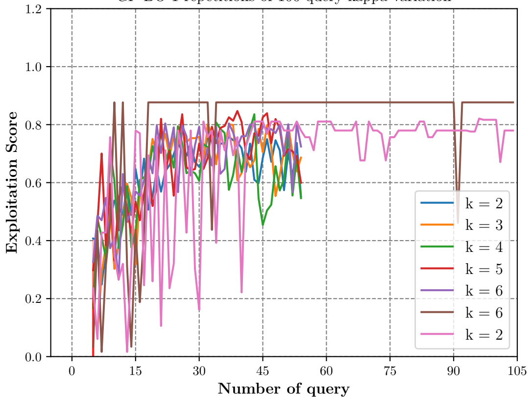
GP-BO 1 repetitions of 100 query kappa variation
